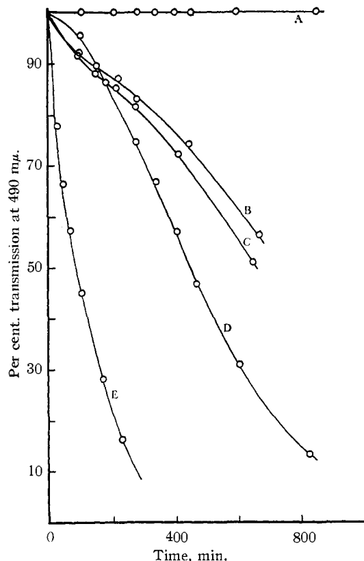
Fig. 6.—Rate of change in the percentage transmission at 490 mμ of D-glucose and 5-(hydroxymethyl)-2-furaldehyde in the presence and absence of glycine; 0.2500 molar (in each constituent) aqueous solutions at reflux temperature (102°): Curve A, D-glucose alone; B, D-glucose and 5-(hydroxymethyl)-2-furaldehyde; C, 5-(hydroxymethyl)-2-furaldehyde alone; D, D-glucose and glycine; E, 5-(hydroxymethyl)-2-furaldehyde and glycine; Lumetron (Mod. 402E) photoelectric colorimeter.
